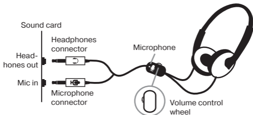
Fig. 1. Connection diagram
